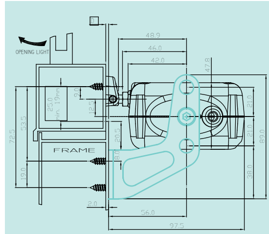
ACK4LPB - Large Pivot Bracket
