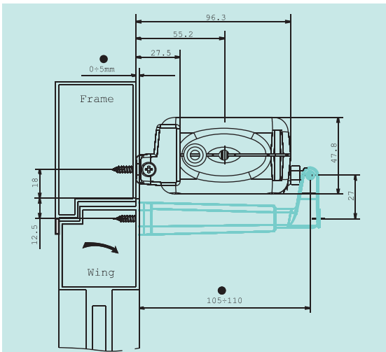
ACK4BHB - Bottom-Hung Bracket
