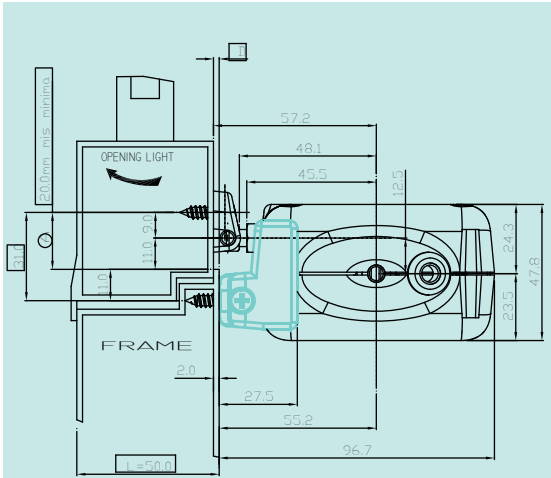
ACK4SB - Standard Bracket
