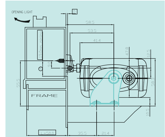
ACK4SPB - Small Pivot Bracket
