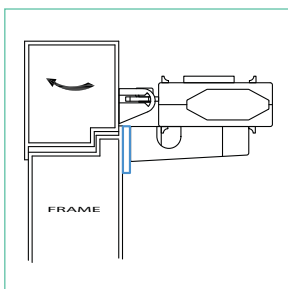
T740 Narrow Fixing Plate for Aluminium frames
