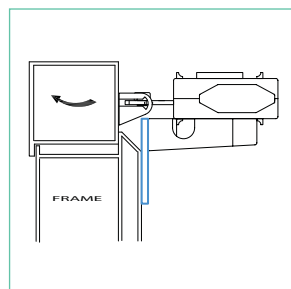
T750 Wide Fixing Plate for PVCU frames
