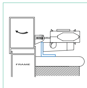
T760 Angled Fixing Plate for Timber frames
