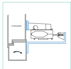
T850 Bottom-Hung Fixing Kit
